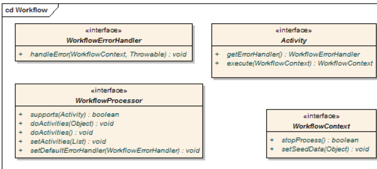
Figure 2.1. Workflow API
