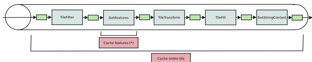
Figure 1.1. Cache interceptors in the GetVectorTile pipeline
