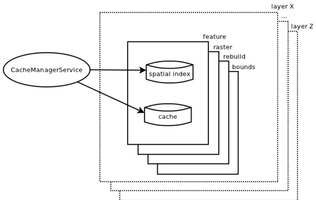
Figure 1.3. CacheManager and cache per layer and category
