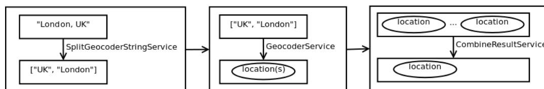
Figure 1.1. GetLocationForStringCommand overview
