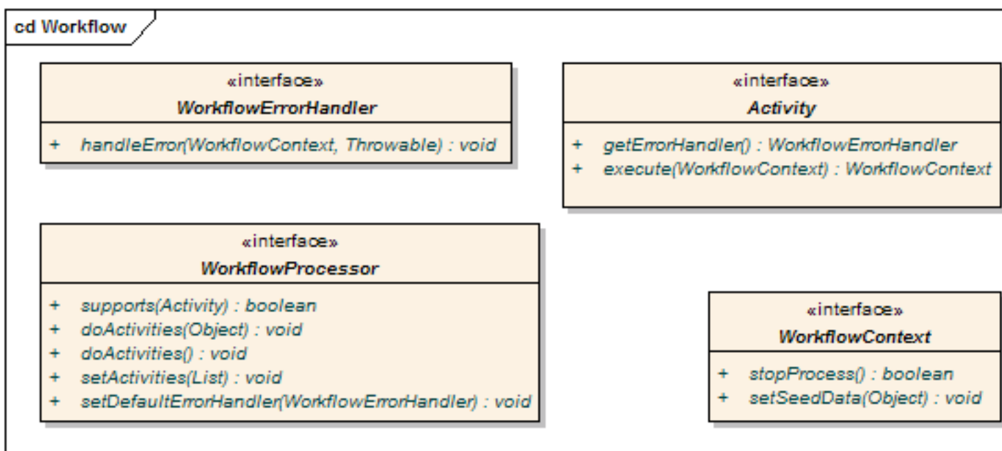
Figure 2.1. Workflow API
